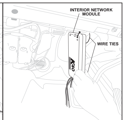
VERTICAL MOUNT
