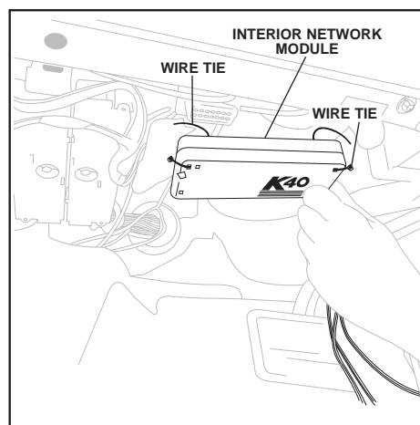
HORIZONTAL MOUNT
